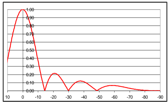
8 Bay elevation pattern
